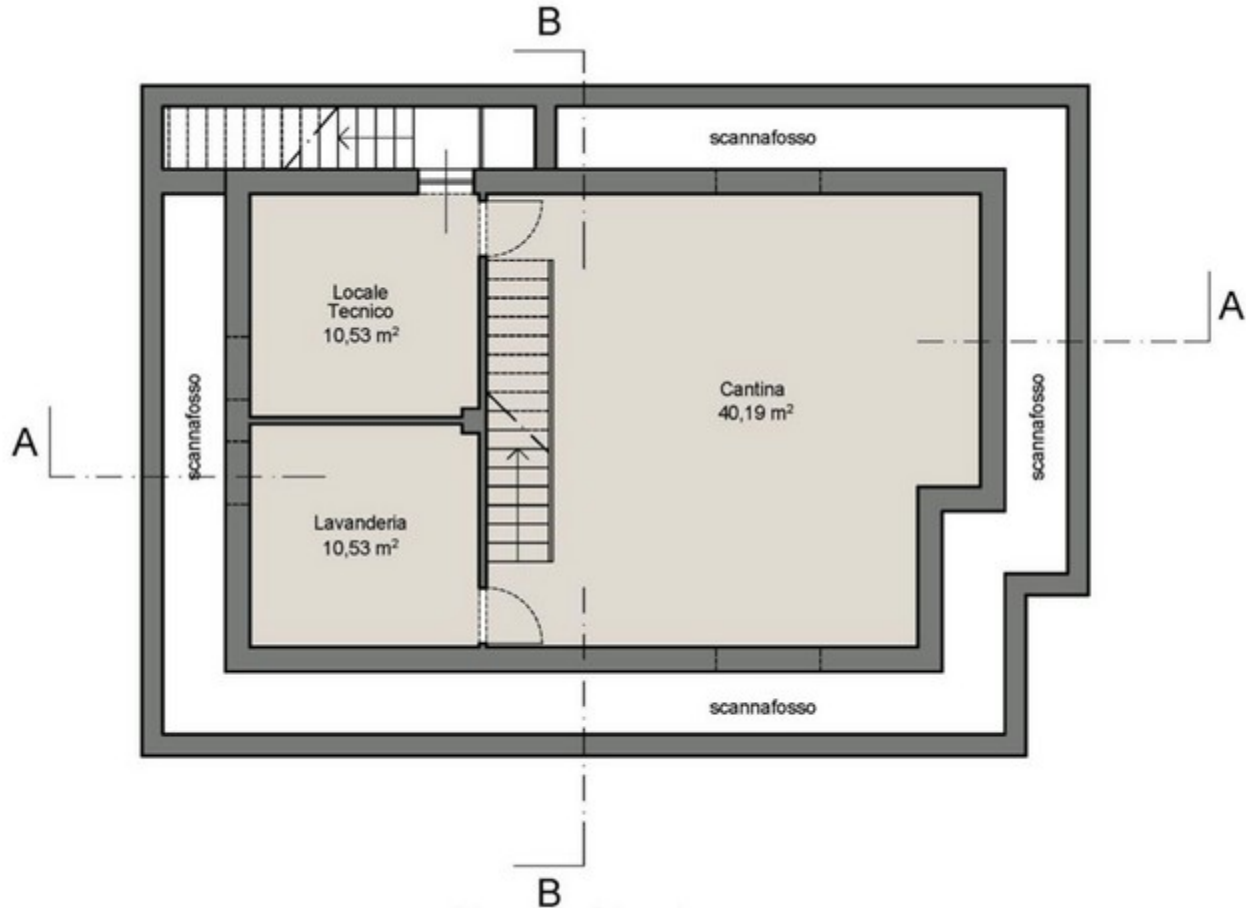
Piano Seminterrato
